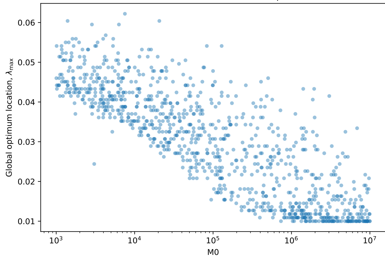
M0 versus location of the fitness optimum
