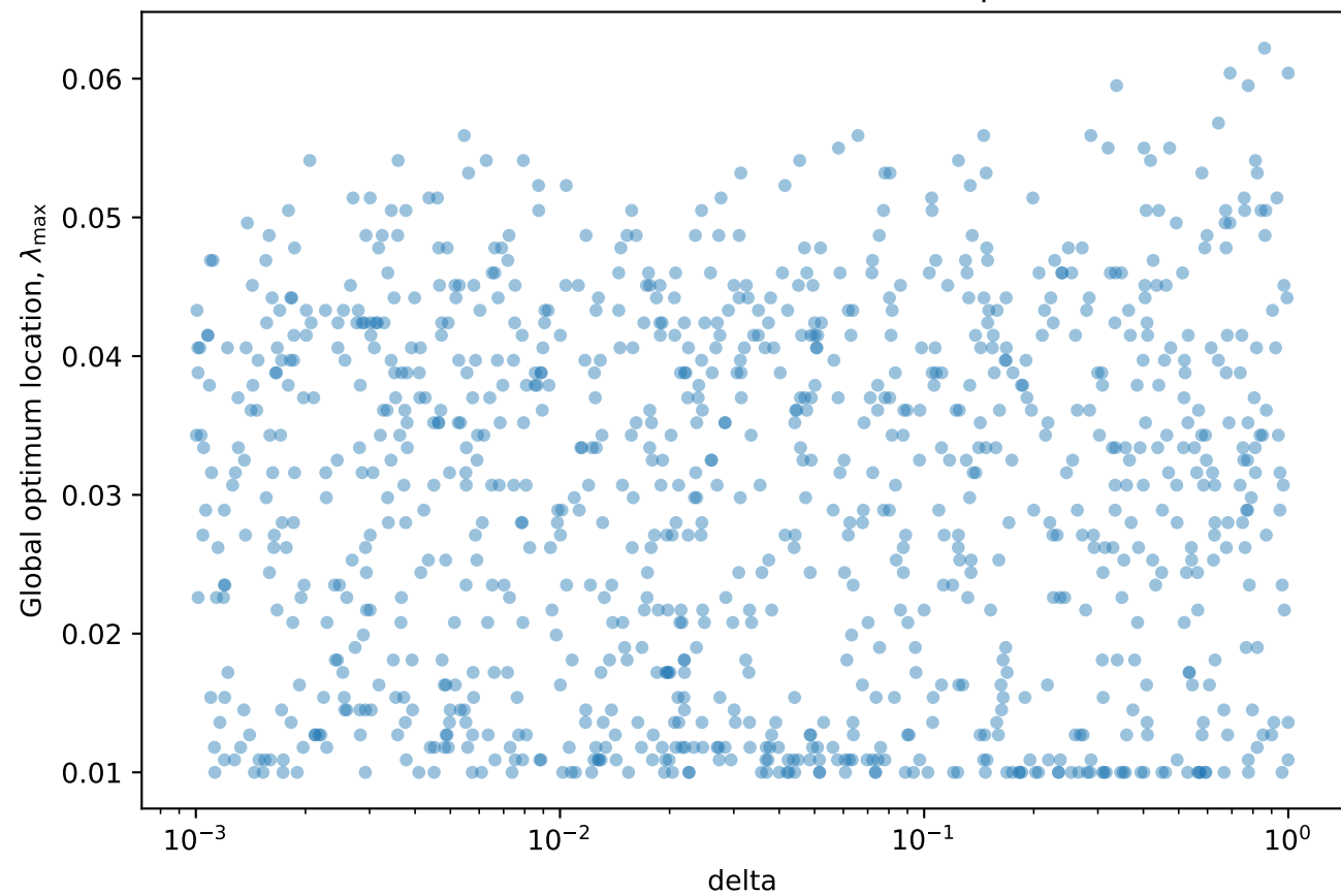
delta versus location of the fitness optimum
