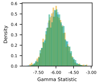
Gamma Statistic
