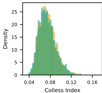
Colless Index
