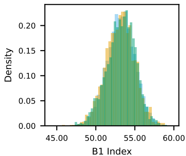
B1 Index
