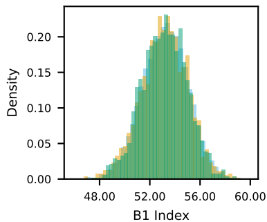
B1 Index
