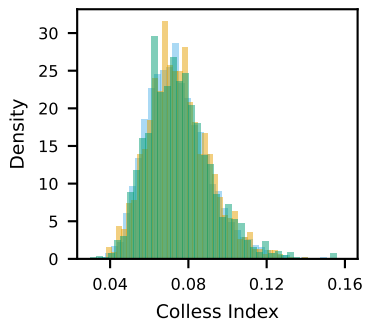
Colless Index
