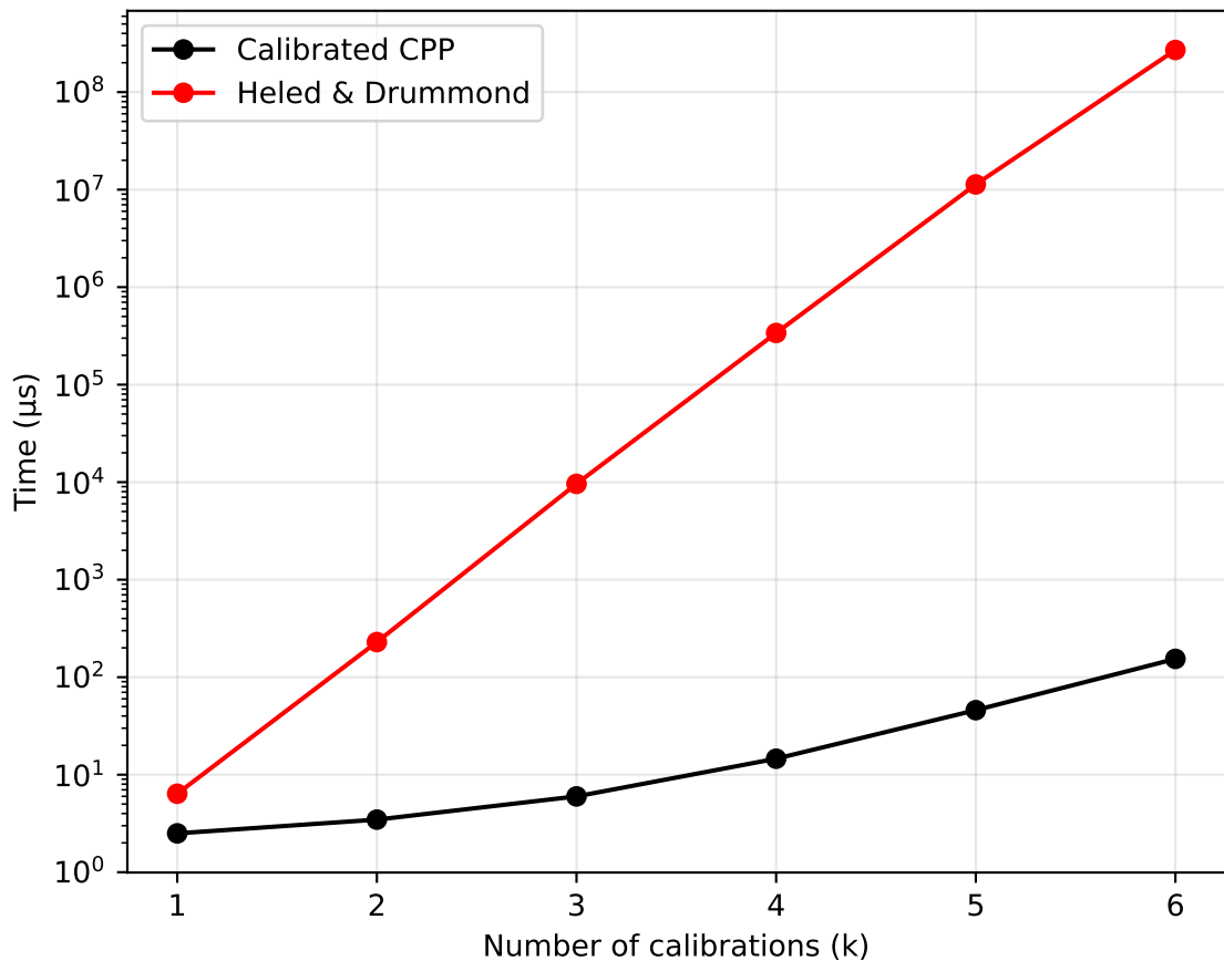
Likelihood Calculation Time
