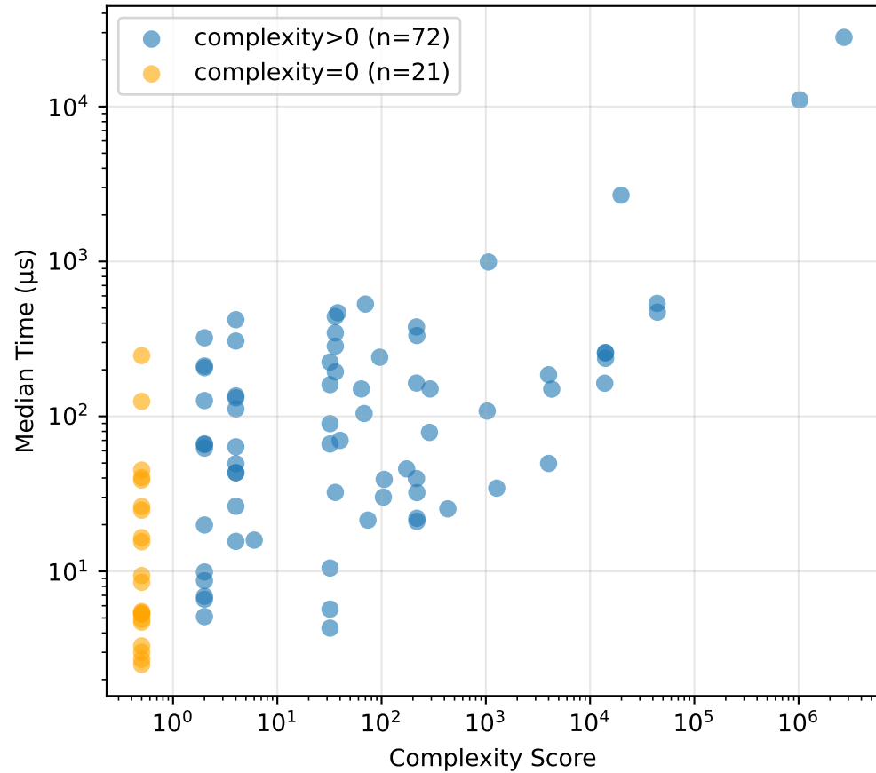
Time vs Complexity (Log-Log)
