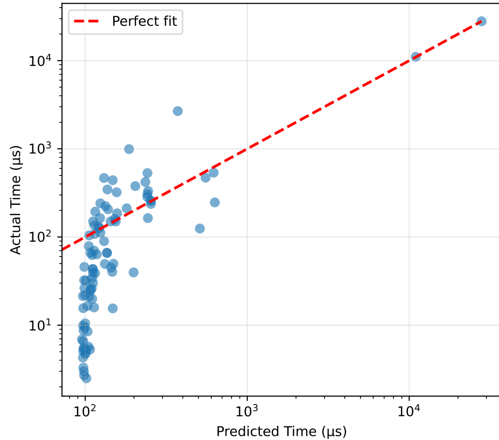
Multivariate Fit ( R^2=0.9919 )
