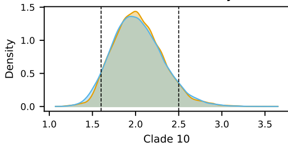
Clade 10 BEAST=0.894 LPhy=0.876
