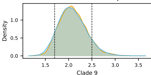
Clade 9 BEAST=0.833 LPhy=0.824
