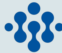
Wwise
