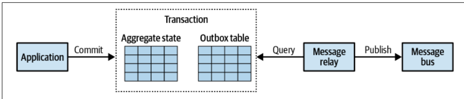
Figure 9-12. Outbox table
