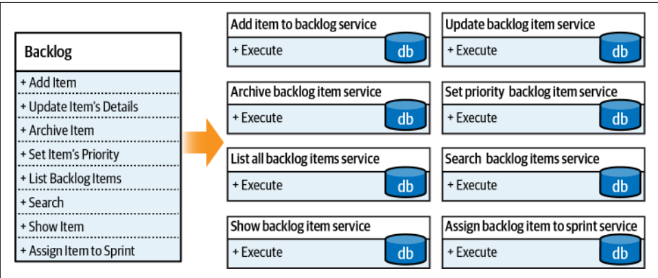
Figure 14-3. Naïve decomposition
