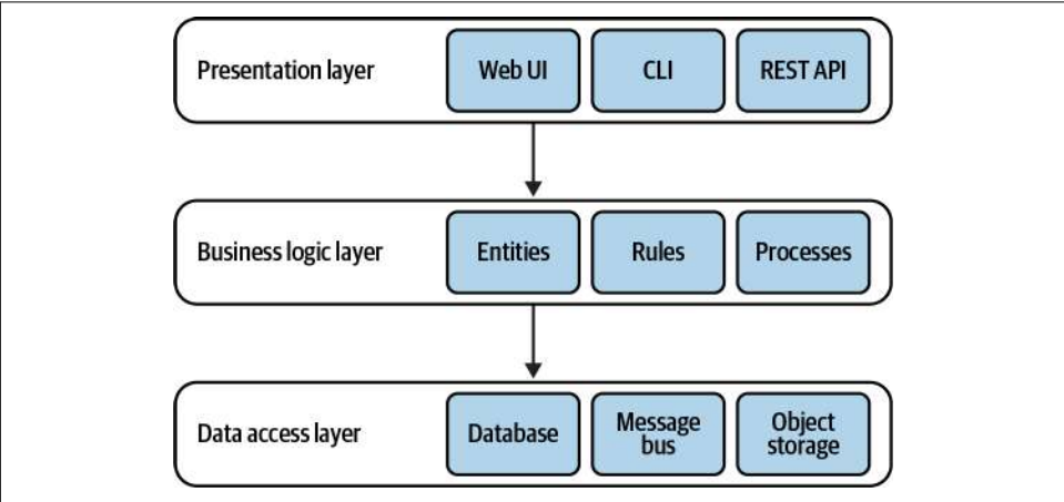
Figure 8-5. Layered architecture
