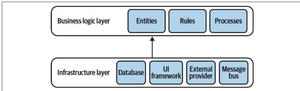
Figure 8-9. Reversed dependencies
