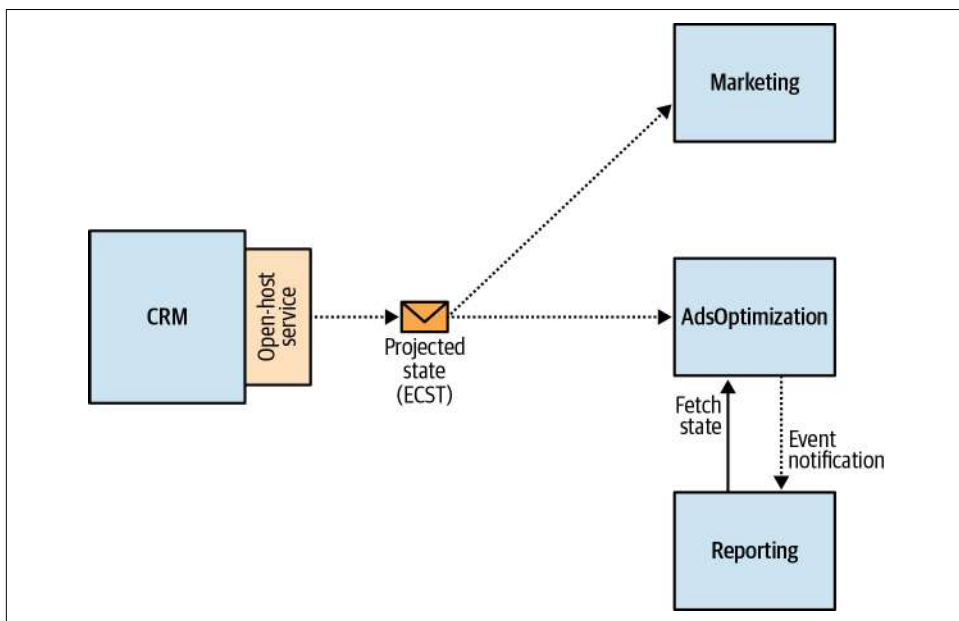
Figure 15-6. Refactored system
