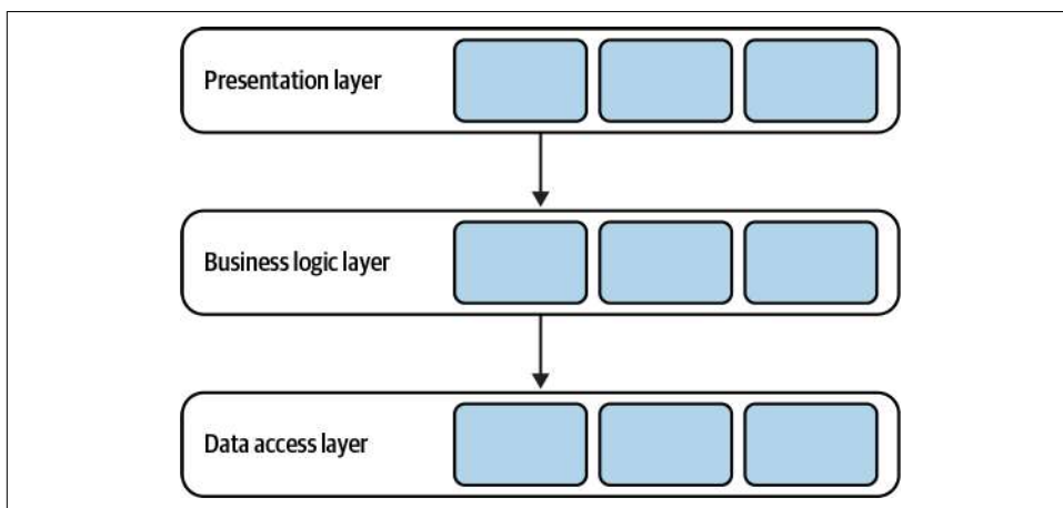
Figure 8-1. Layered architecture
