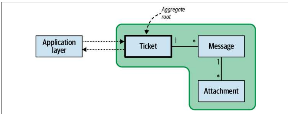
Figure 6-5. Aggregate root
