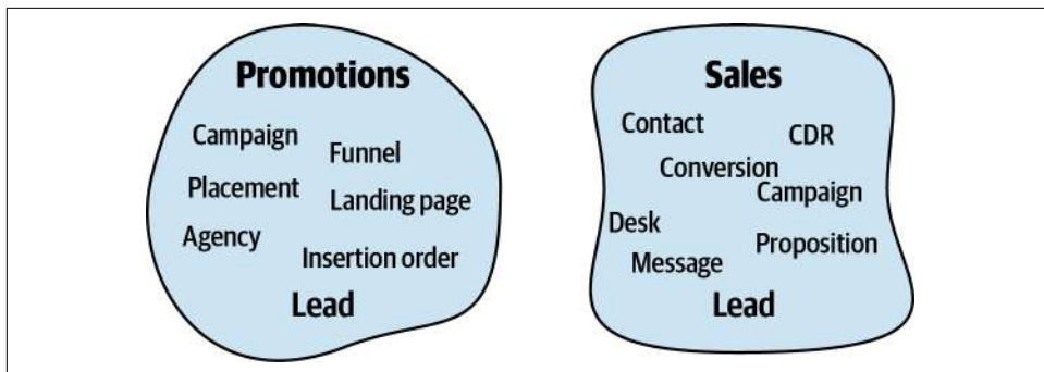
Figure 14-8. Bounded contexts
