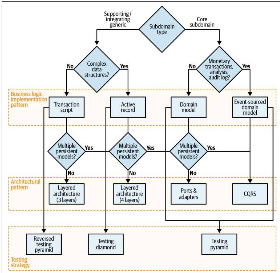
Figure E-1. Decision tree summarizing heuristics for tactical decision-making
