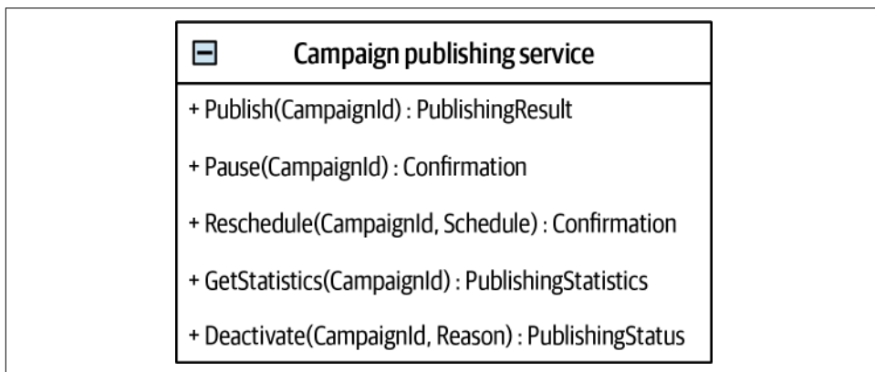
Figure 14-2. A service's public interface
