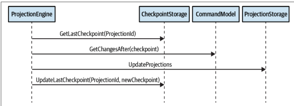
Figure 8-14. Synchronous projection of read models through catch-up subscription
