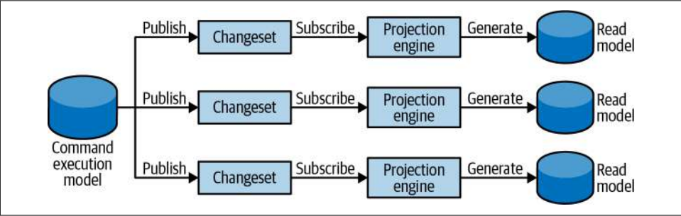
Figure 8-16. Asynchronous projection of read models
