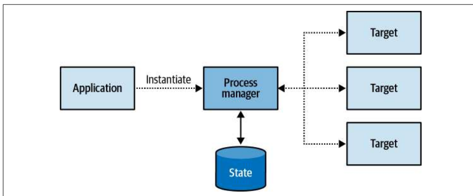
Figure 9-14. Process manager
