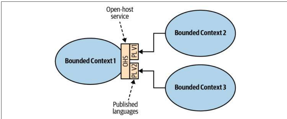
Figure 4-7. Open-host service exposing multiple versions of the published language
