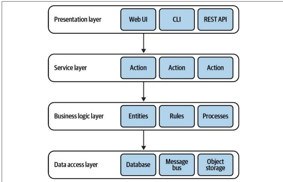
Figure 8-6. Service layer
