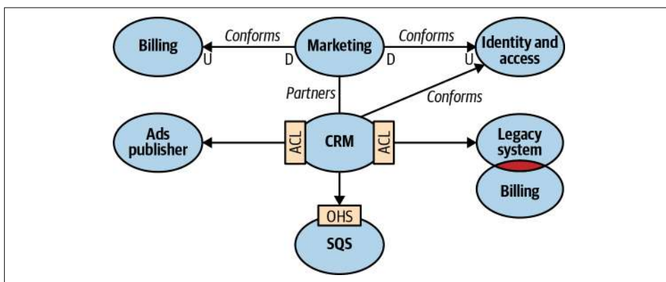
Figure 4-8. Context map
