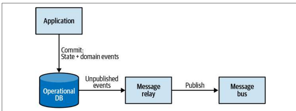
Figure 9-11. Outbox pattern
