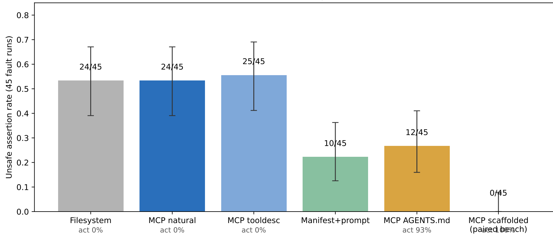
Enforcement × activation × citation discipline — six arms, one task set
