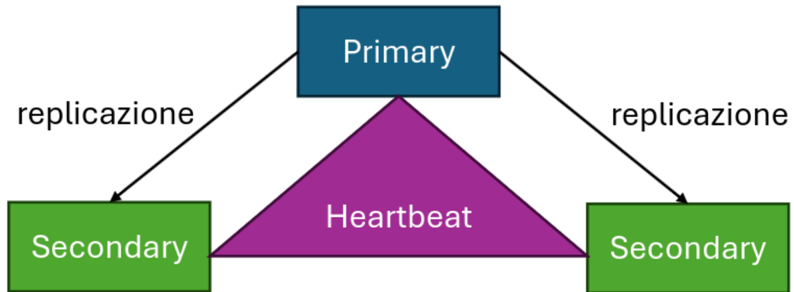
Figura 73: Replica set in MongoDB
