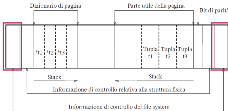
Figura 35: Block header e block trailer
