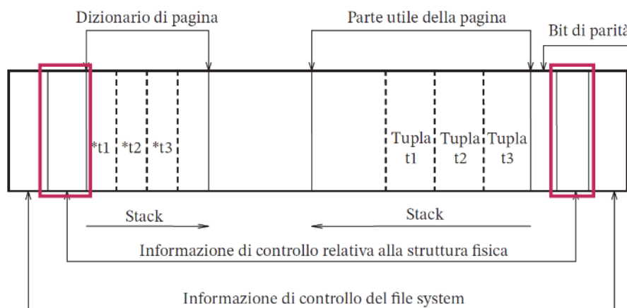
Figura 36: Page header e page trailer
