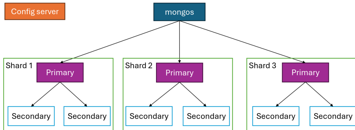
Figura 74: Sharding in MongoDB
