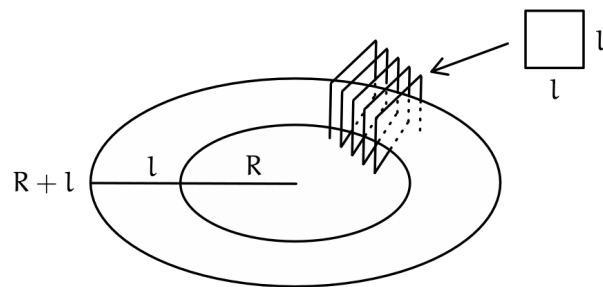
Figura 171: Solenoide toroidale
