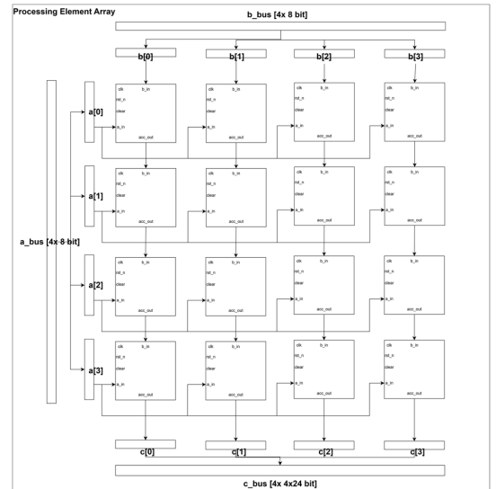
Fig. 4. Processing element array.
