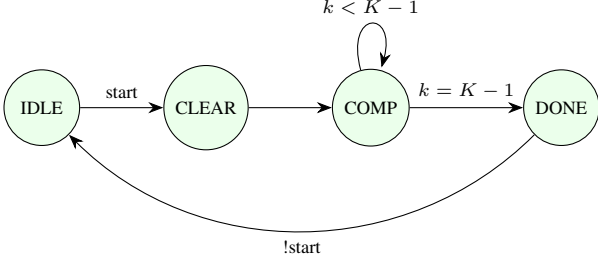
Fig. 5. Controller state machine.
