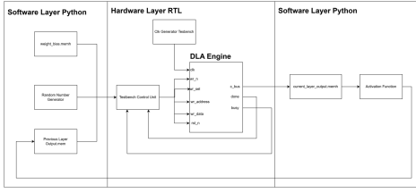
Fig. 7. Hardware and software flow.
