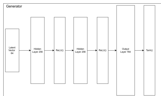
Fig. 1. GAN generator layer architecture.
