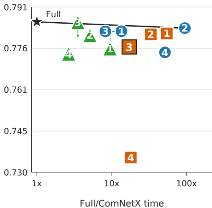
dyn_pubmed
