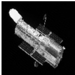
TSVD RRE=0.0474
