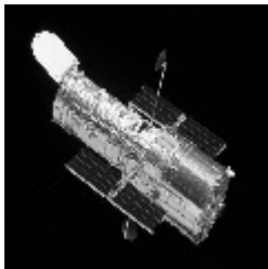
RBD RRE=0.0487
