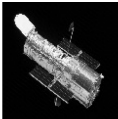
SOC RRE=0.0486
