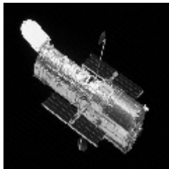
SEC RRE=0.0486
