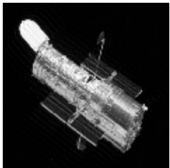
MM-GKS (25) RRE=0.1129
