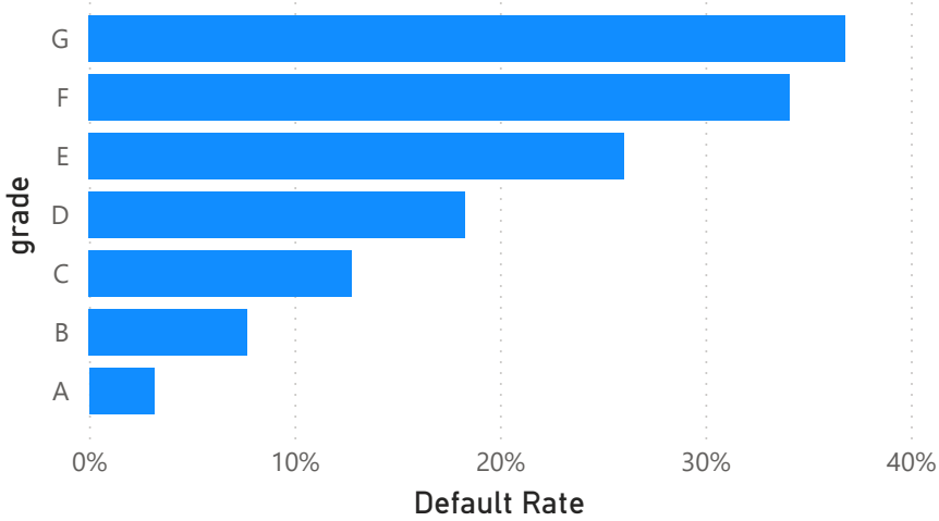
Default Rate by grade
