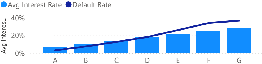
Avg Interest Rate and Default Rate by grade
