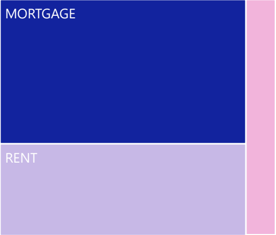
Total Disbursed by home_ownership
