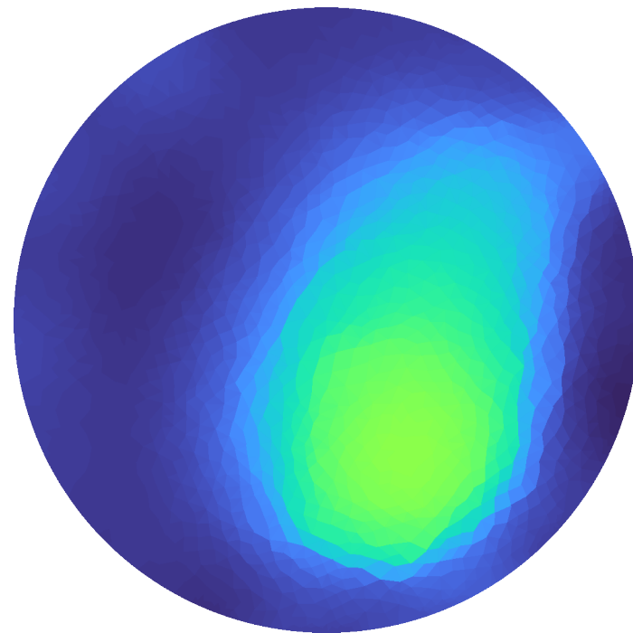
Iteration 2
