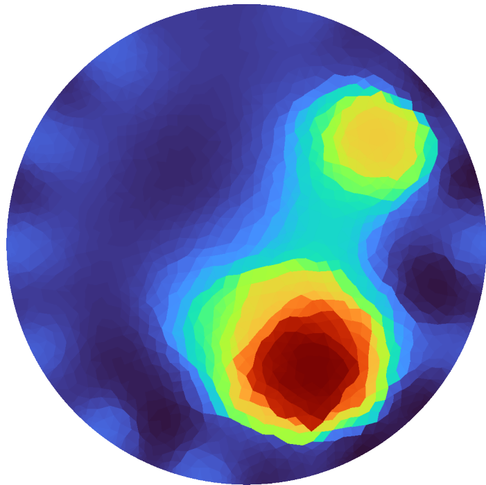
Iteration 5
