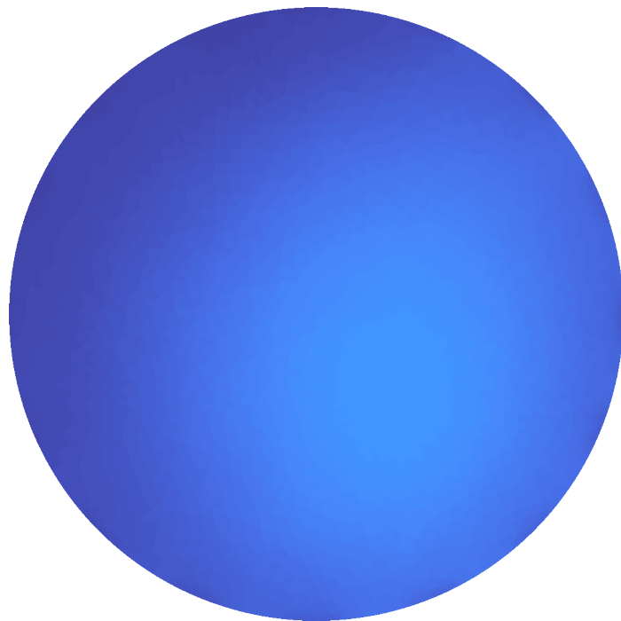
Iteration 1
