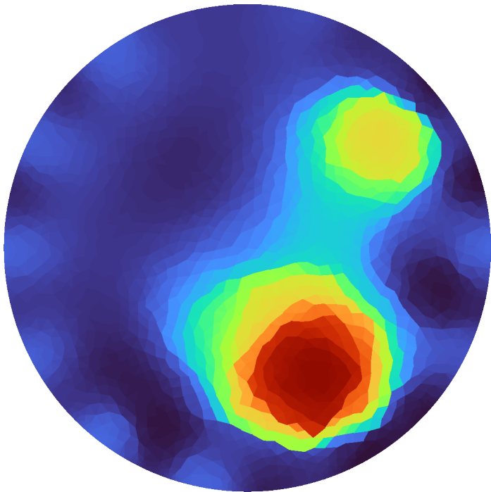
Iteration 4
