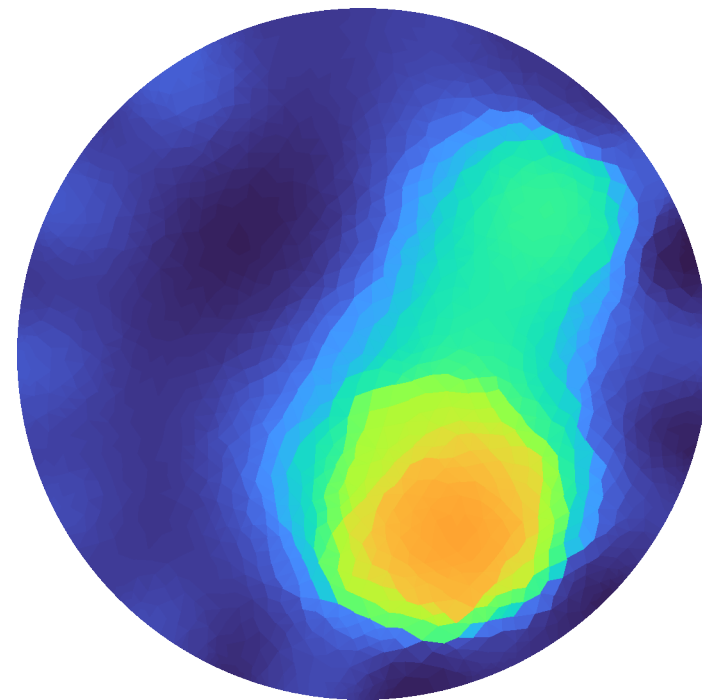
Iteration 3
