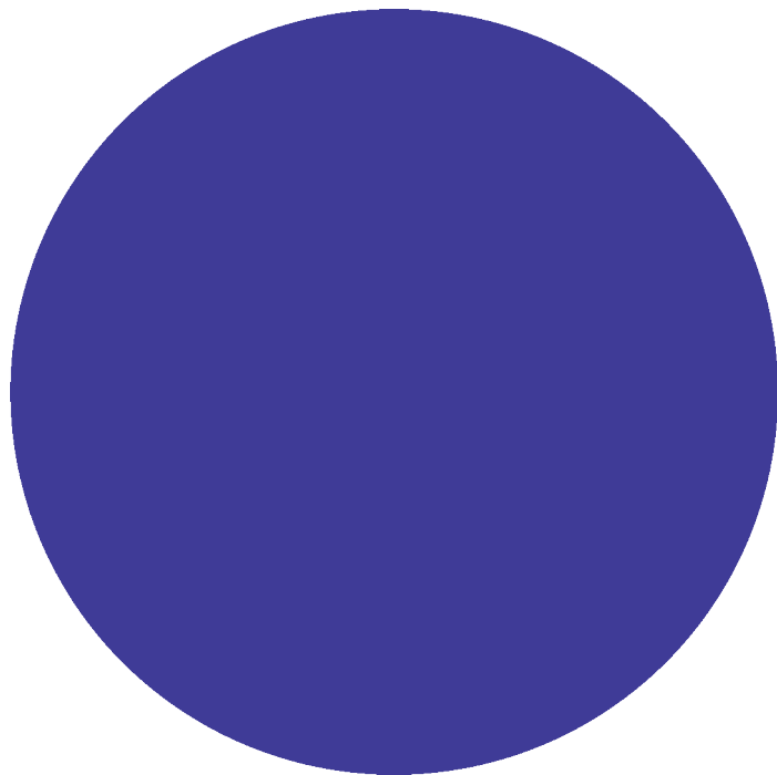
Iteration 0
