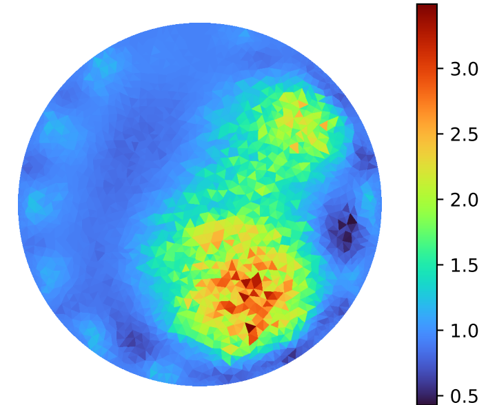
Iteration 4
