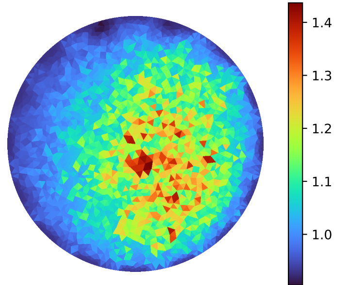
Iteration 1
