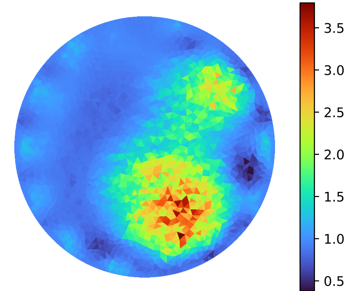
Iteration 5
