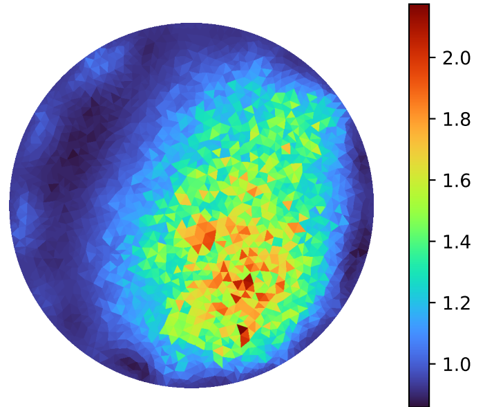
Iteration 2
