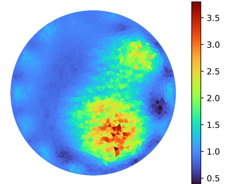
Iteration 6
