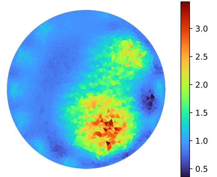
Iteration 3
