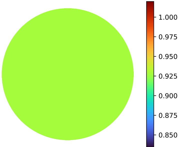
Iteration 0
