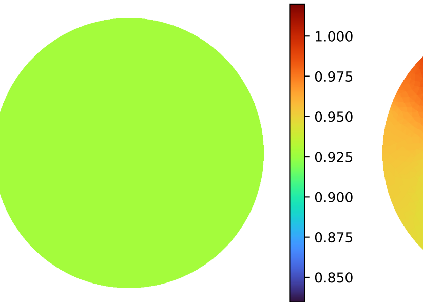
Iteration 0
