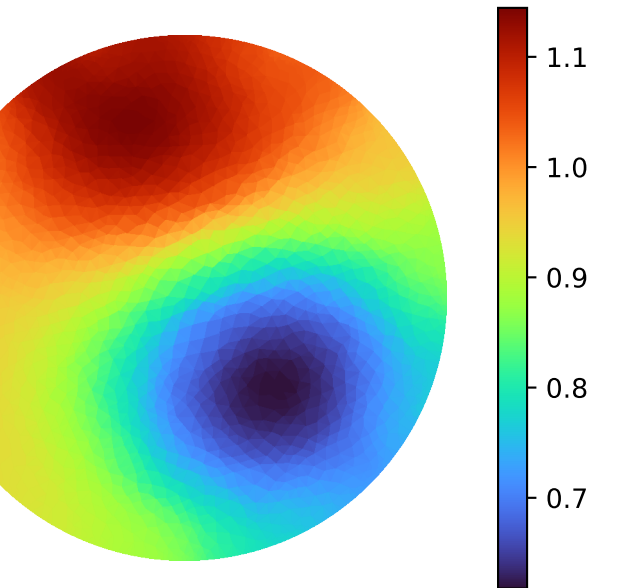
Iteration 1
