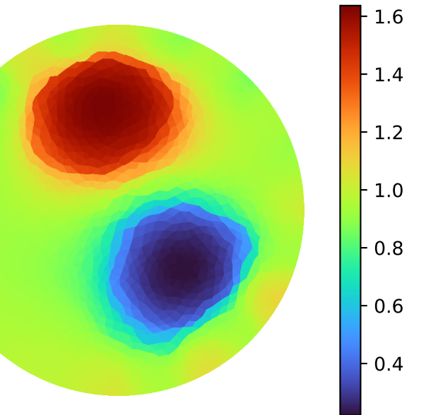
Iteration 3
