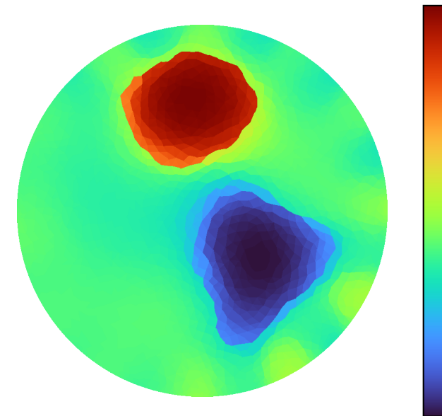
Iteration 5
