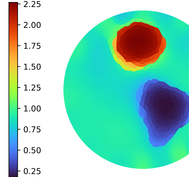
Iteration 7
