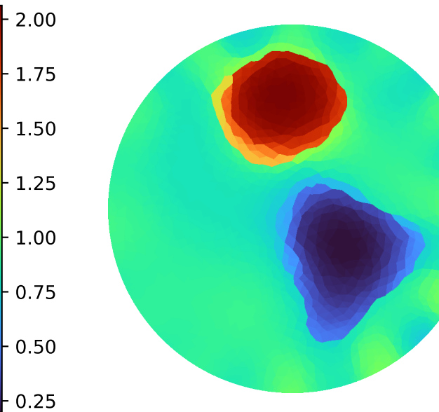
Iteration 6
