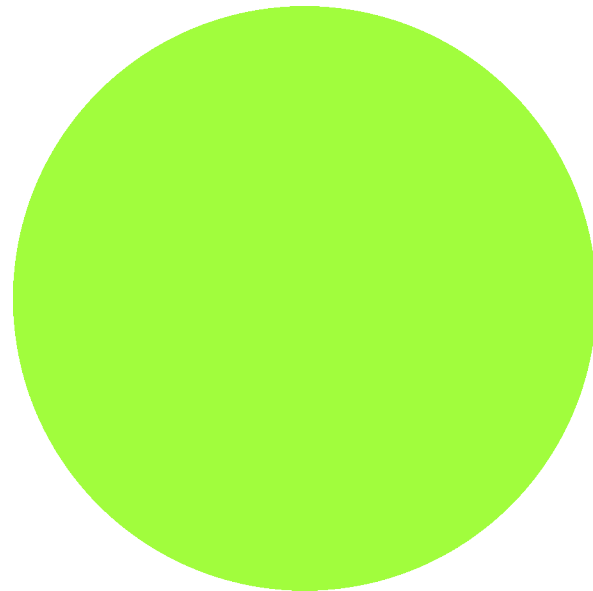
Iteration 0
