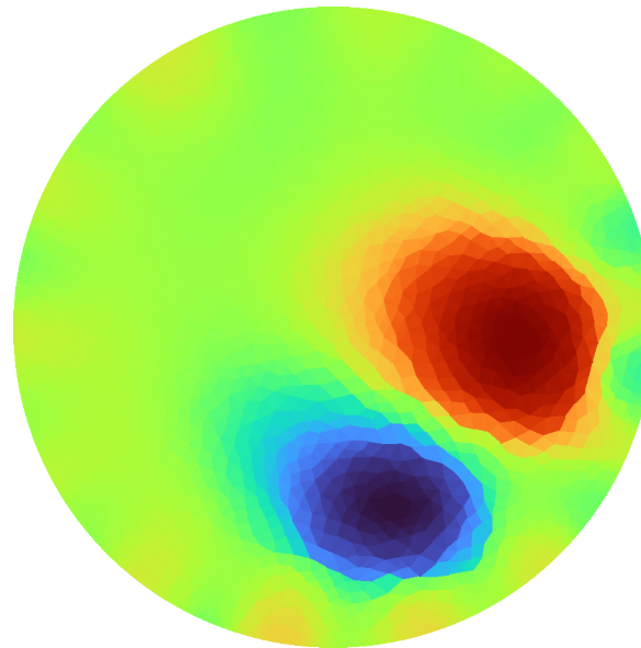
Iteration 2
