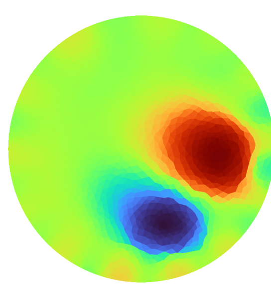
Iteration 3
