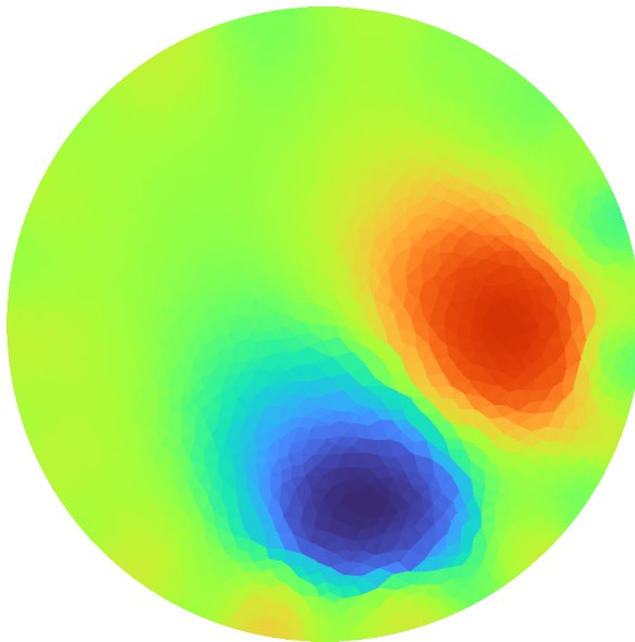
Iteration 1
