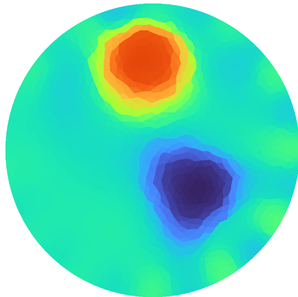
Method 2
