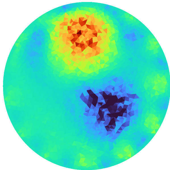
Method 1
