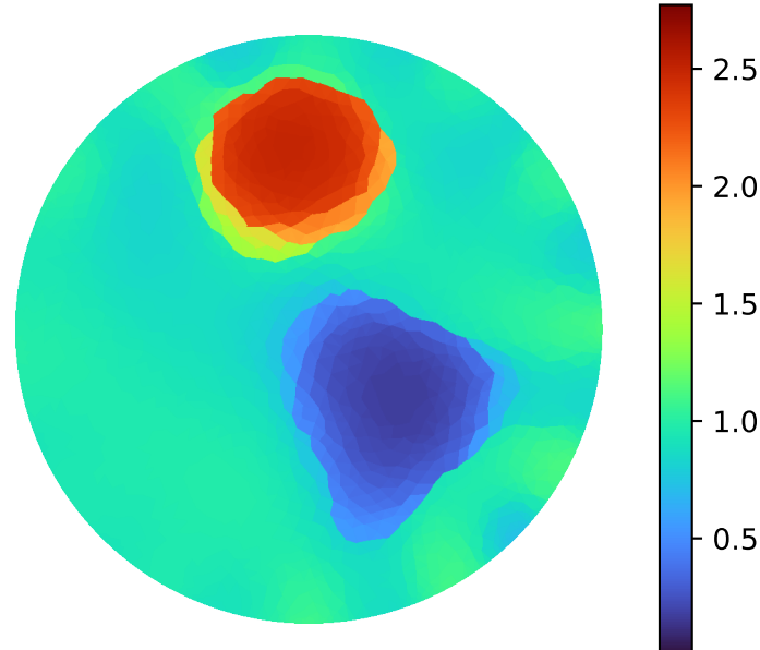
Method 3
