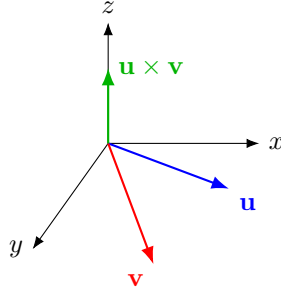
Figure 8: Cross product
