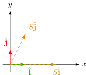
Figure 10: Eigenvectors and Eigenvalues
