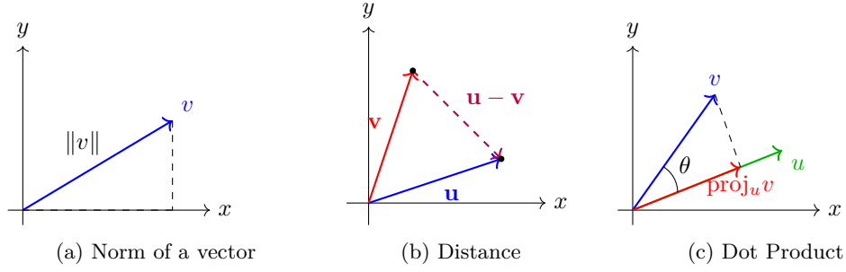
Figure 9: Norm and Dot Product
