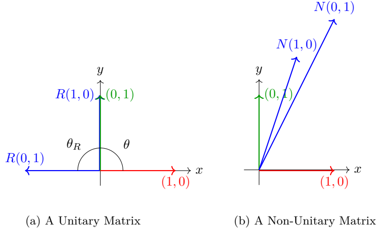
Figure 12: Unitary and Non-Unitary Matrices
