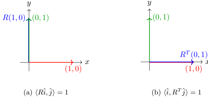
Figure 11: Hermitian adjoint
