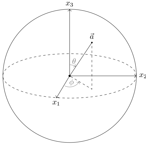
Figure 14: Bloch Sphere
