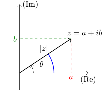
Figure 16: A geometric representation of complex numbers.
