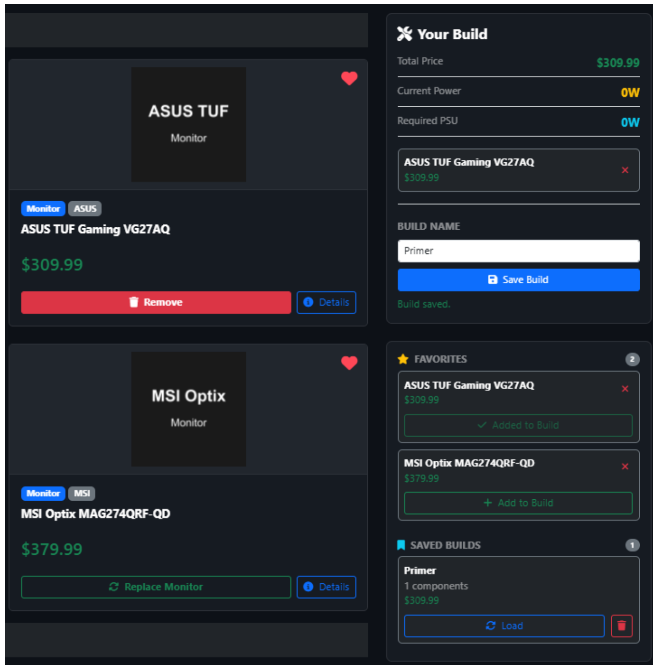
Slika 6. Saved builds
