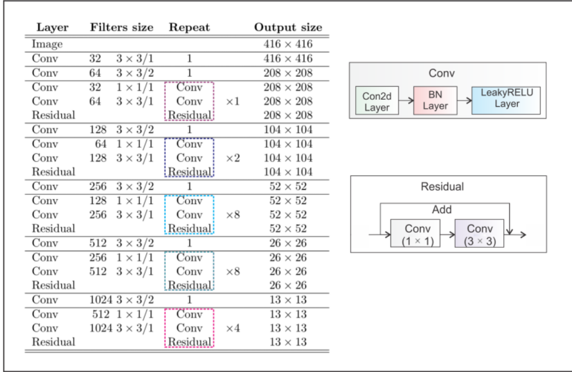
Figure 8.10: yolo v3 architecture
