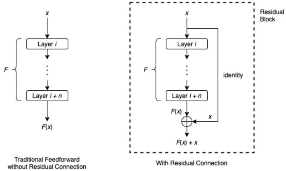
Figure 7.1: residual connection diagram
