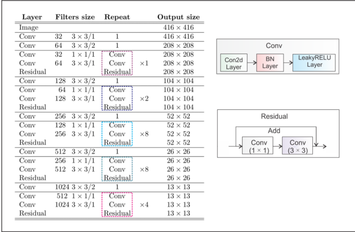
Figure 6.10: yolo v3 architecture
