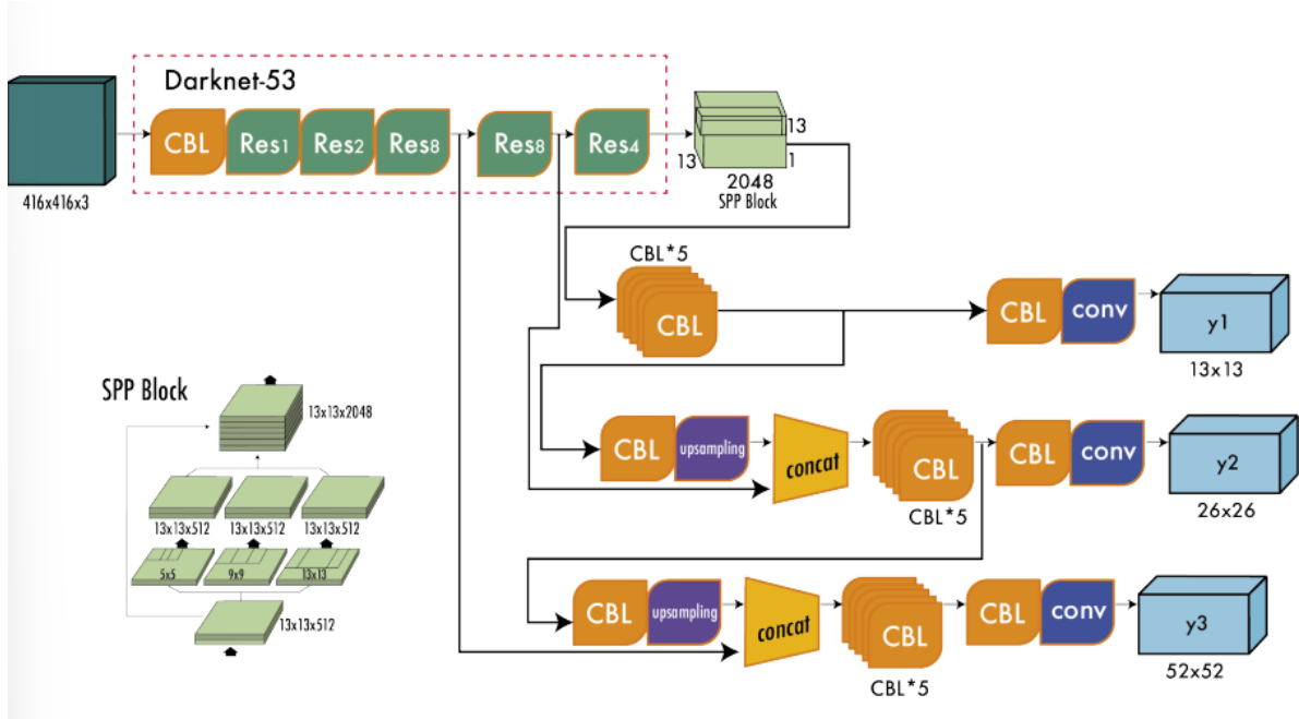
Figure 6.11: darknet 53 backbone
