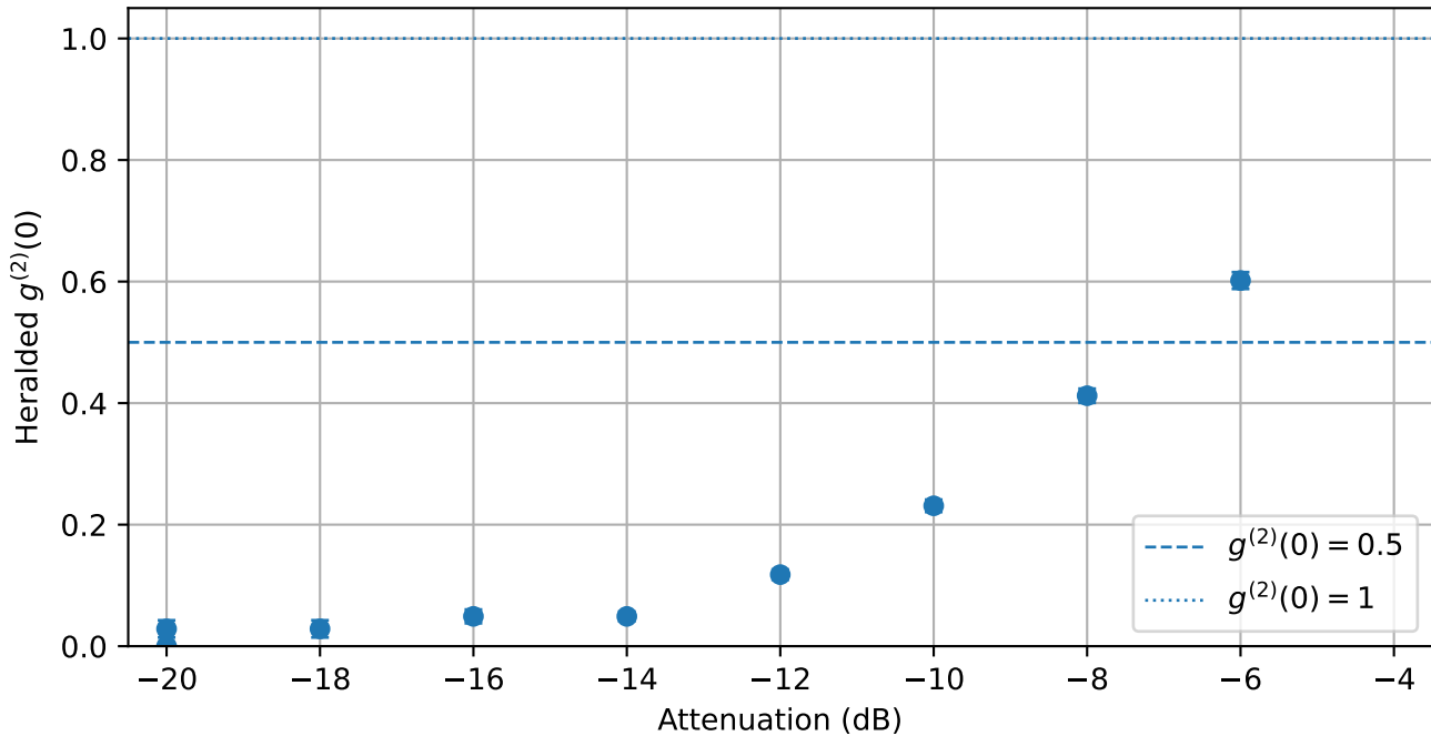
Heralded g^{(2)}(0) vs attenuation (CH3 herald)
