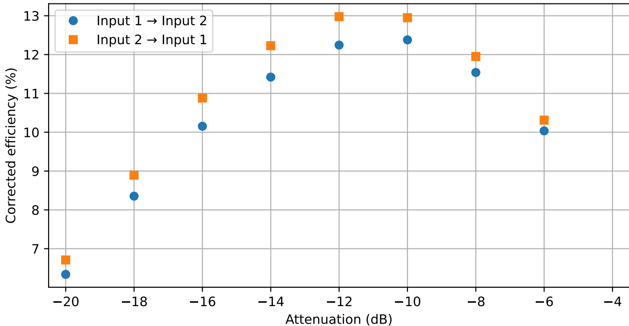
Corrected heralded efficiency vs attenuation
