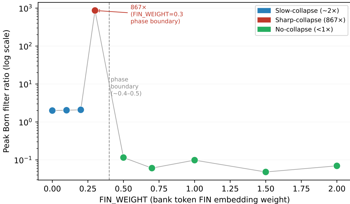
Born filter three-regime phase diagram (G-054) Controlled G-track geometry — NOT T5-small production model Source: findings/METHODS_REPORT_G054.md
