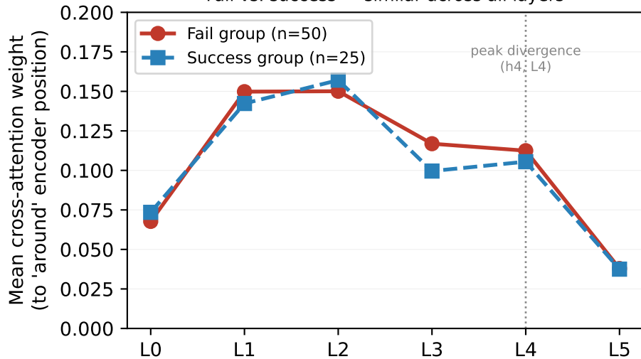
(A) Per-layer attention weight profile Fail vs. success — similar across all layers
