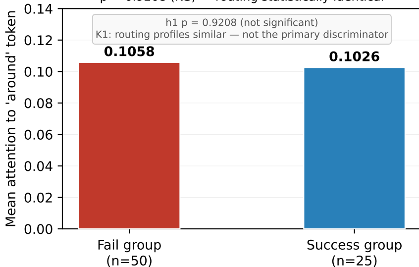
(B) h1: mean attention comparison p = 0.9208 (NS) — routing statistically identical
