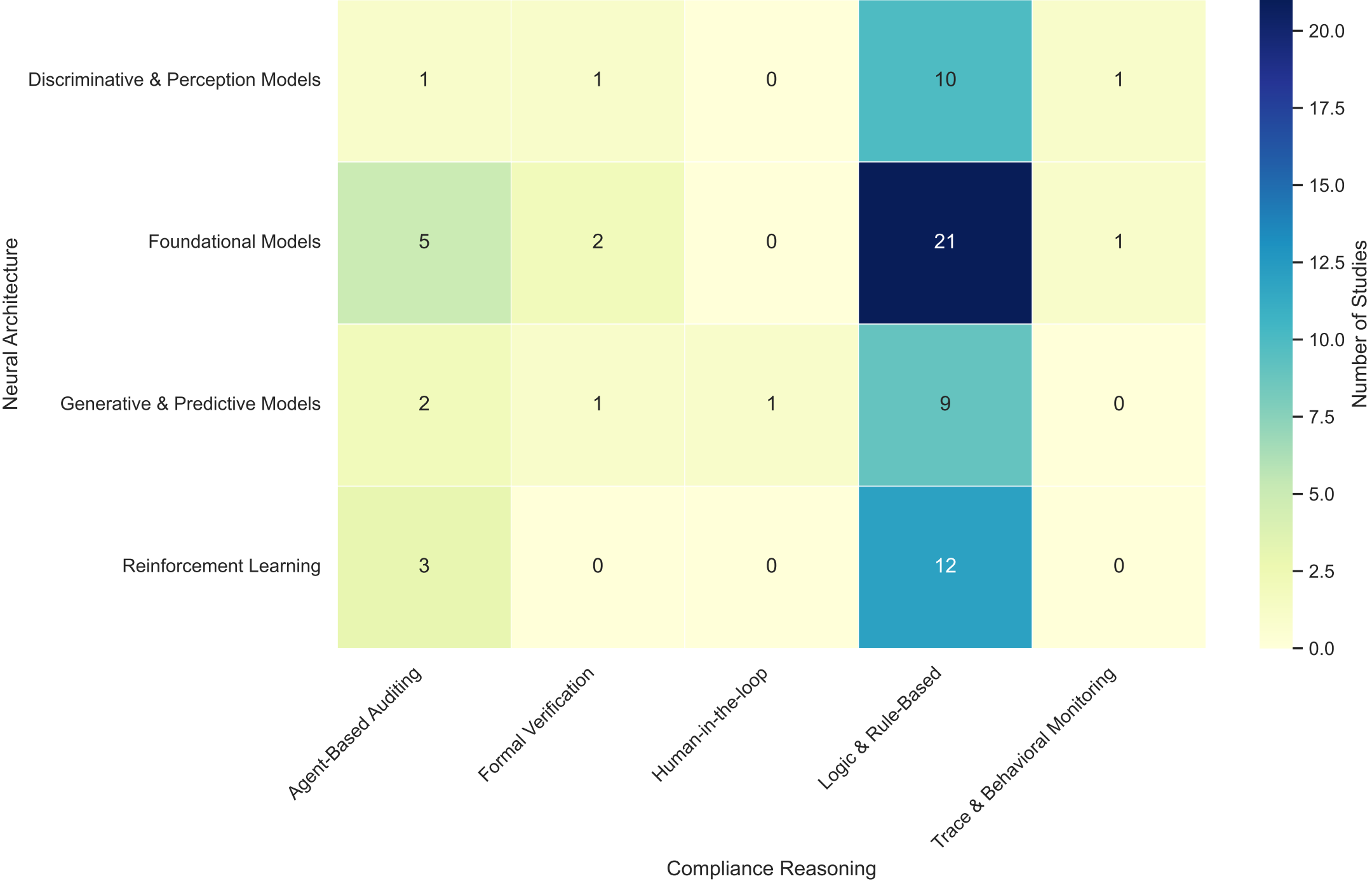
Intersection Analysis: Neural Architectures vs. Compliance Reasoning (Absolute)
