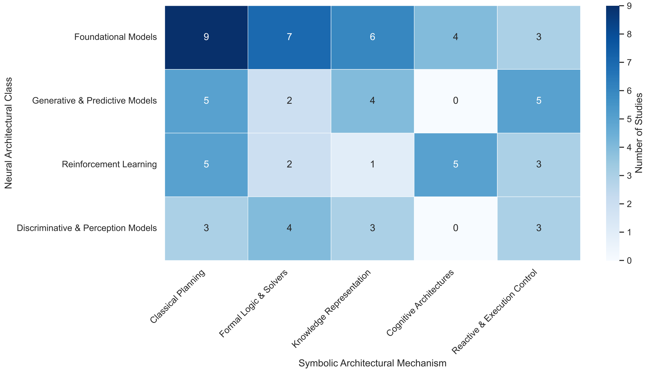
Intersection Analysis: Neural Classes vs. Symbolic Mechanisms
