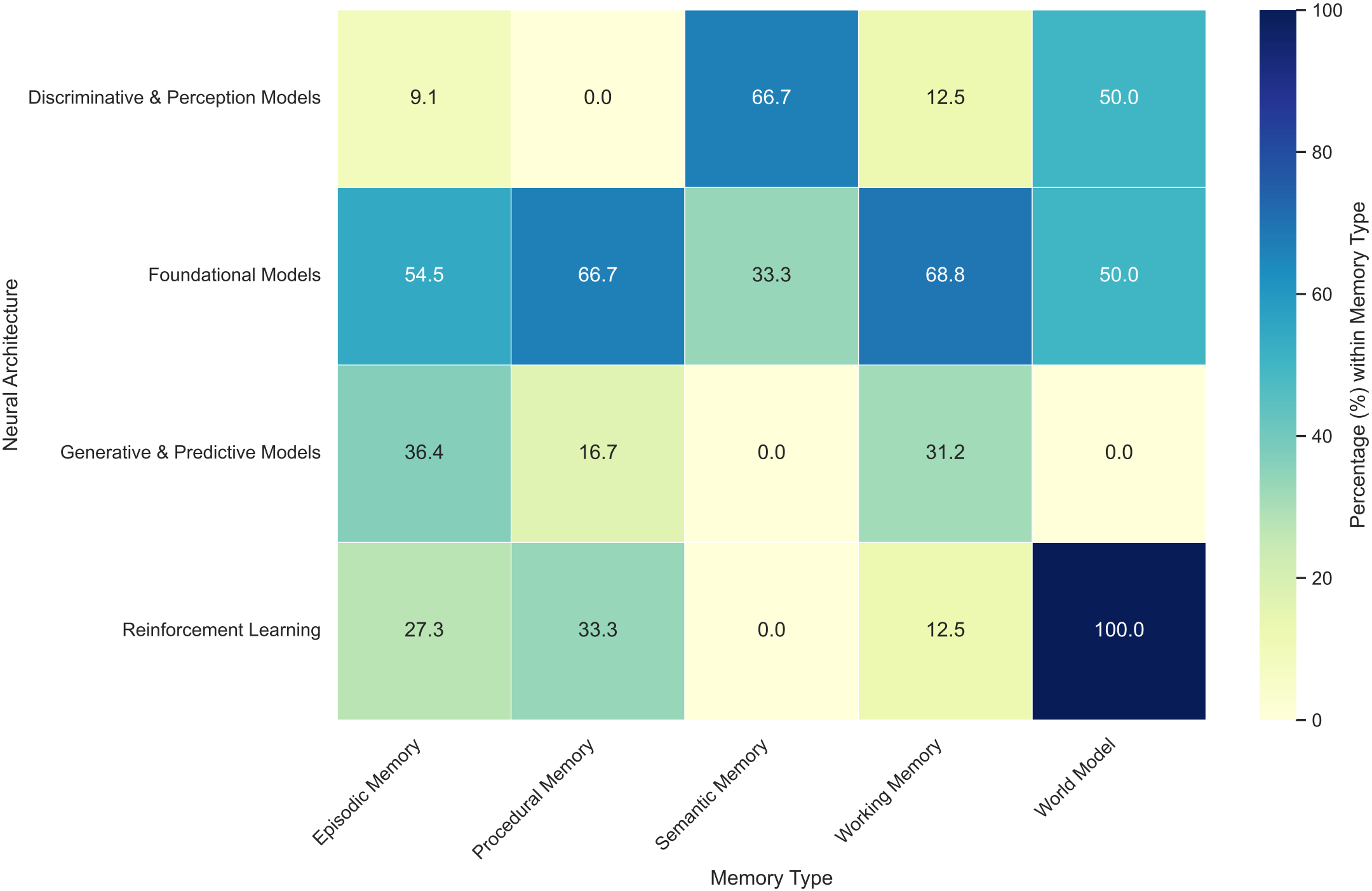
Intersection Analysis: Neural Architectures vs. Memory Types (Normalized)
