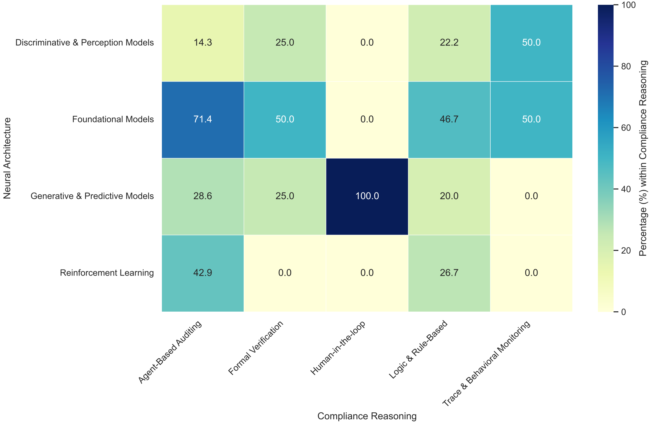
Intersection Analysis: Neural Architectures vs. Compliance Reasoning (Normalized)
