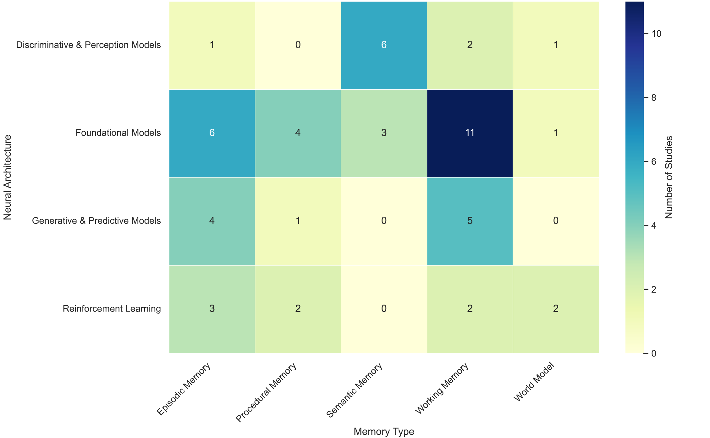
Intersection Analysis: Neural Architectures vs. Memory Types (Absolute)
