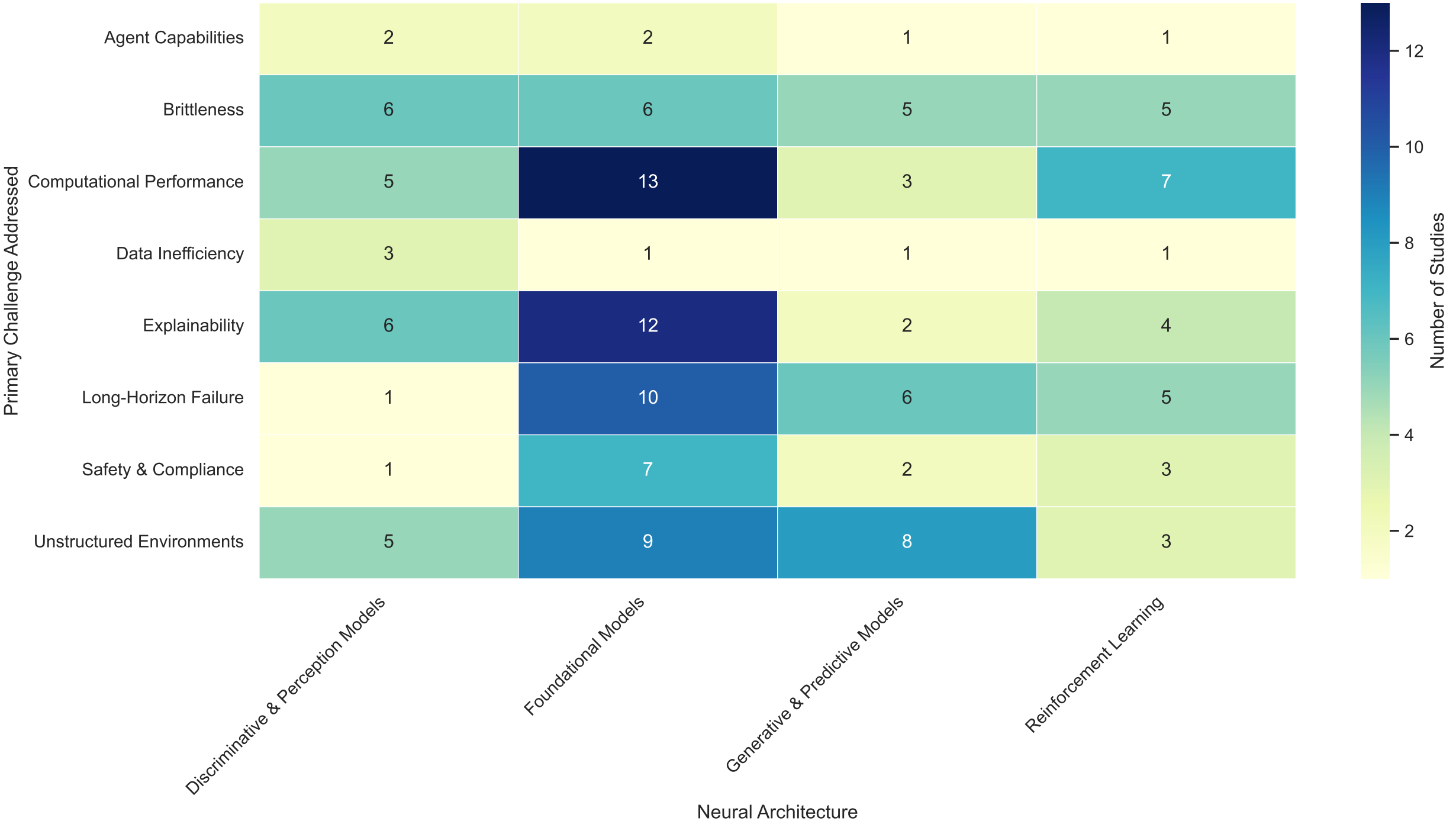
Intersection Analysis: Primary Challenges vs. Neural Architectures (Absolute)
