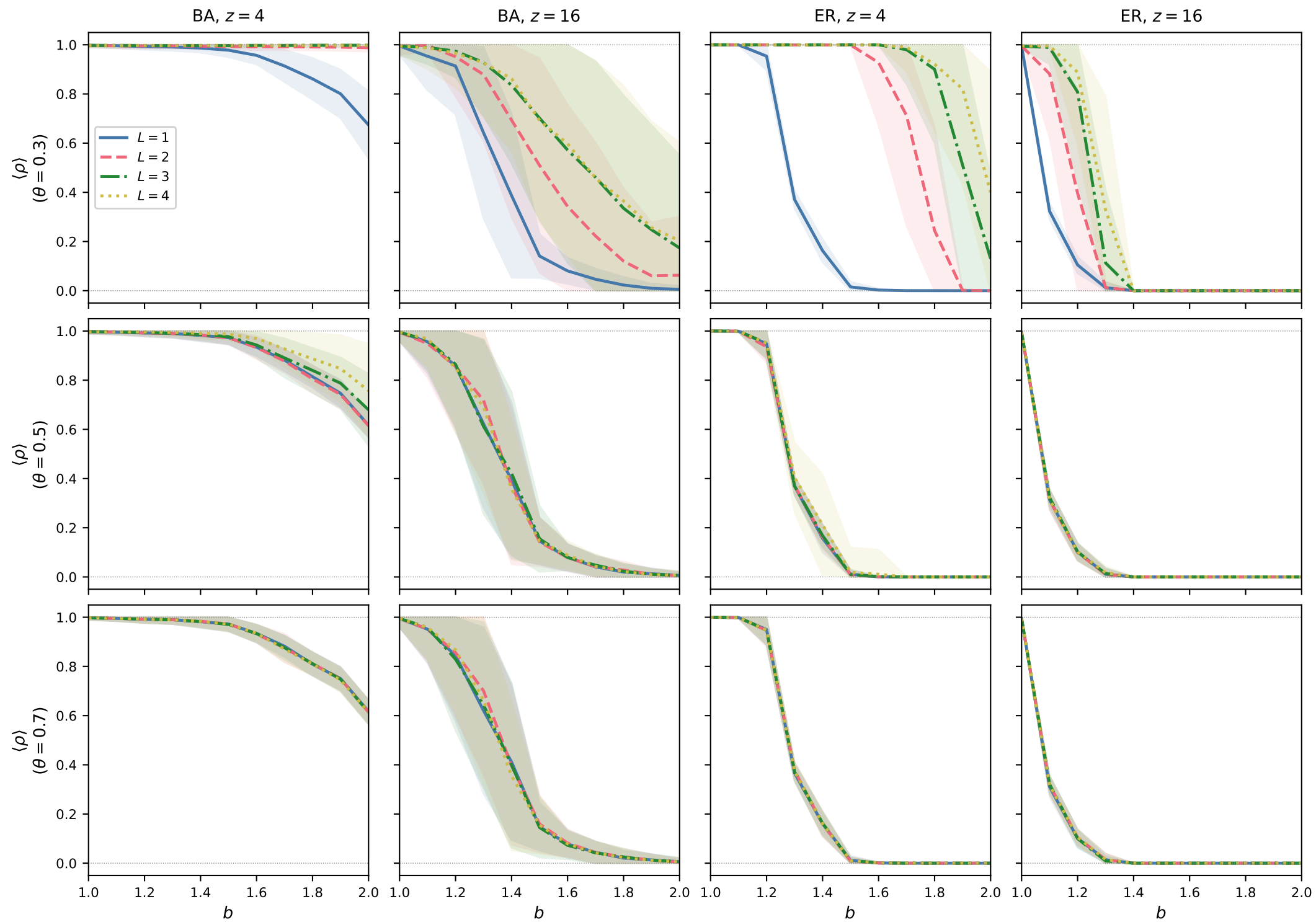
\langle \rho \rangle vs b — effect of L , correlated multiplex
