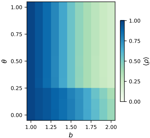
Replicator (PRE 2016)
