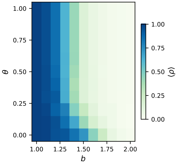
Fermi ( K = 0.1 )
