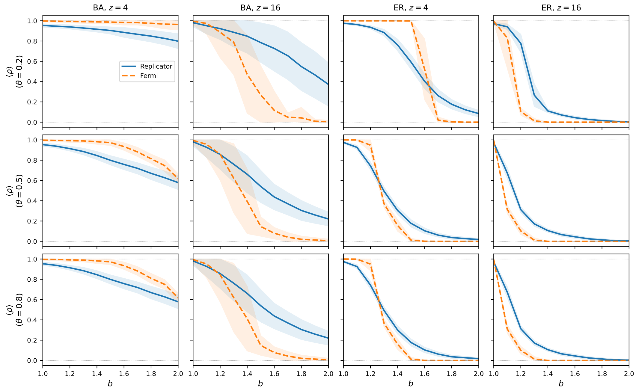
\langle \rho \rangle vs b — REP vs Fermi, L = 1
