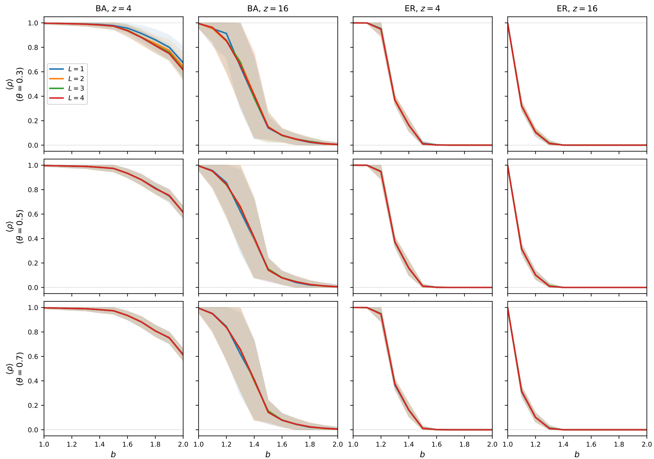
\langle \rho \rangle vs b — effect of L , correlated duplex
