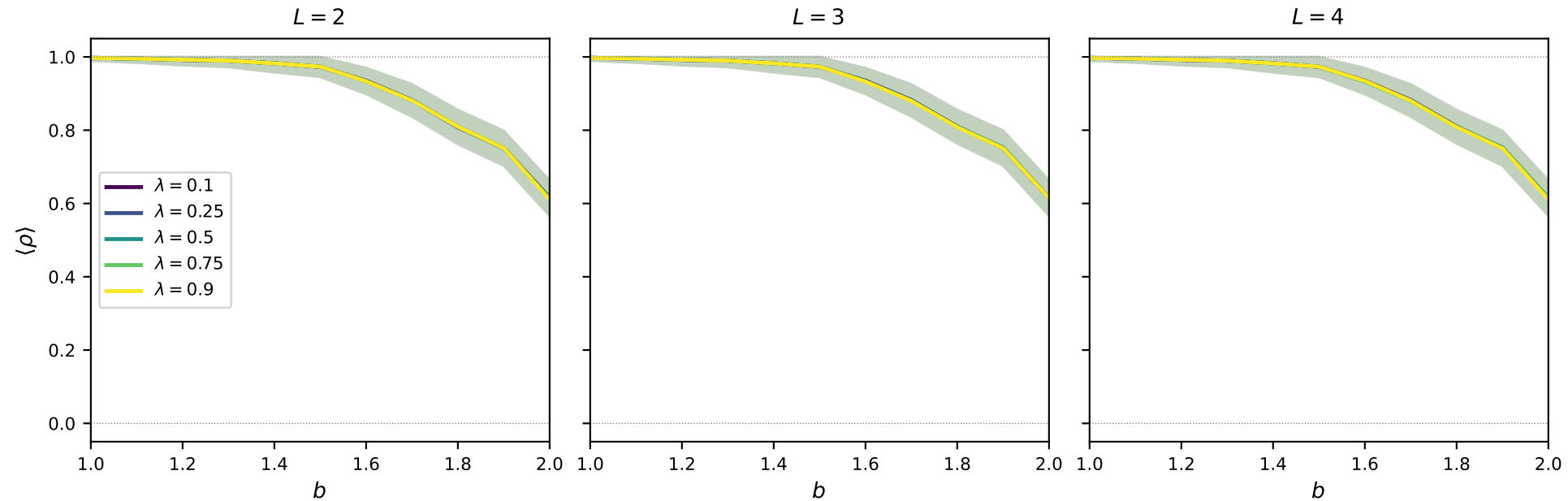
BA, z = 4 — effect of \lambda on \langle \rho \rangle vs b ( \theta = 0.5 )
