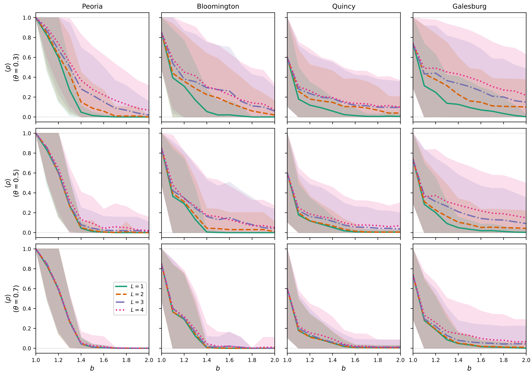
\langle \rho \rangle vs b — effect of L , CKM physician networks
