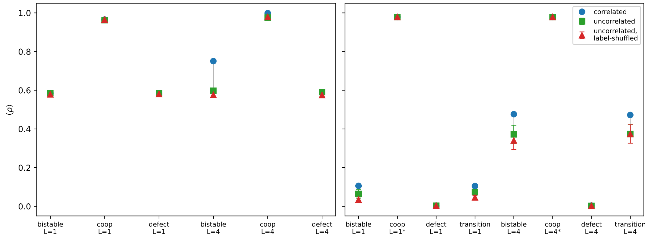
Correlated vs. uncorrelated vs. label-shuffled BA multiplex (* = degenerate point, see text)
