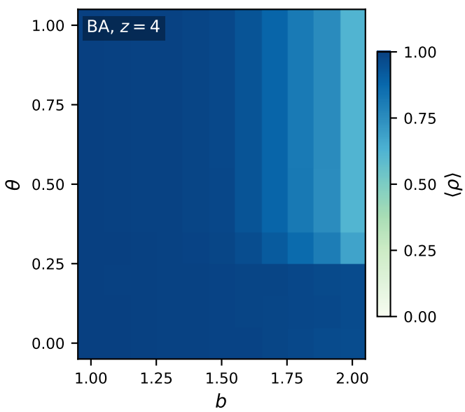
Stationary cooperator fraction — L = 1 , correlated multiplex
