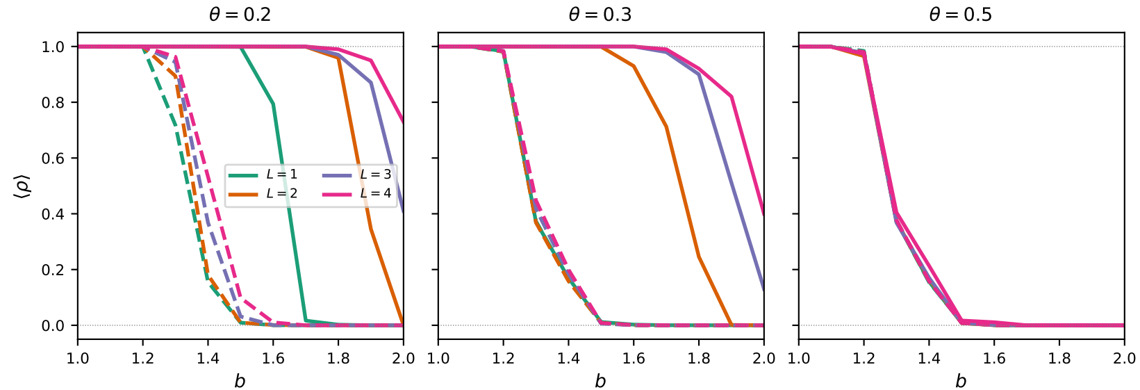
ER z = 4 : correlated (—) vs uncorrelated (- -)
