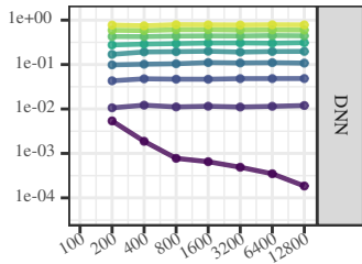
N_{\text{train}} (log 10 scale)
