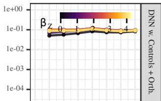
Bias 2 ( \hat{f}_X^{re} ) (log 10 scale)
