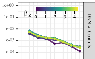
Bias 2 ( \hat{f}_X ) (log 10 scale)
