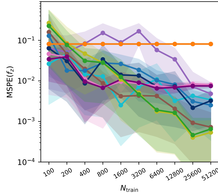
Traffic tabular DGP (cv1=0.8, cv2=0.3): method comparison across N
