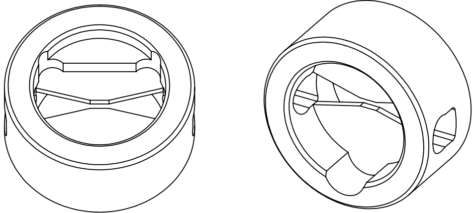
ISOMETRIC VIEWS
