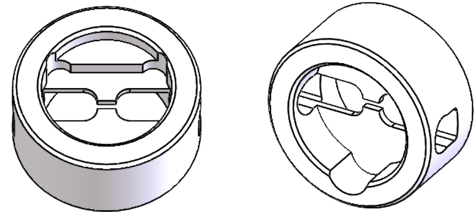
ISOMETRIC VIEWS
