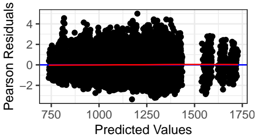
Residual Plot
