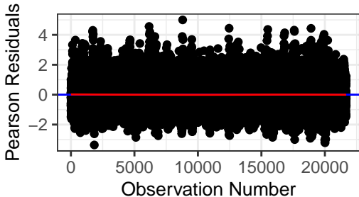
Index Plot
