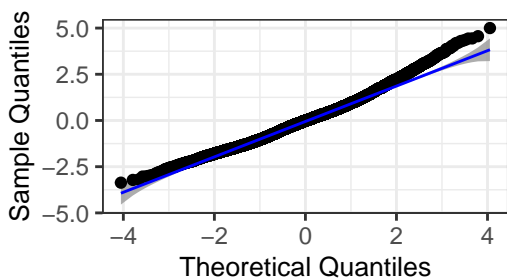
Q-Q Plot
