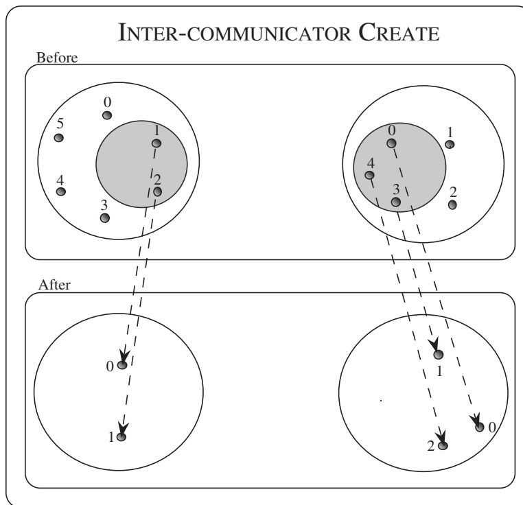
43 Figure 7.1: Inter-communicator creation using MPI_COMM_CREATE extended to inter- 44 communicators. The input groups are those in the grey circle. 45
