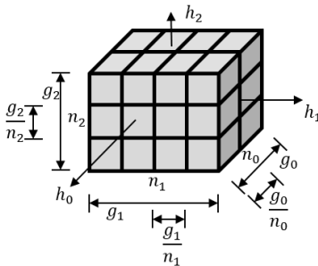
Figure 7.1: Example for the calculation of the weights. The data sizes g_i express the three dimensions of the total application data grid. The virtual process grid dimensions are expressed by n_i . The figure shows the dividing of the total application grid into its subdomains. The value h_i represents the halo width in a given direction when the 2-dimensional side of a subdomain is communicated to the neighbor process in that direction.
