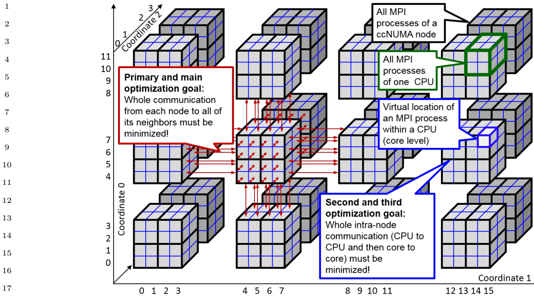
Figure 7.4: Example with 24 nodes (level 0), 4 CPUs per node (level 1) and 8 cores per CPU (level 2). The figure shows the 3-dimensional distribution calculated by MPI_DIMS_ML_CREATE based on weight values (1/12, 1/16, 1/8).
