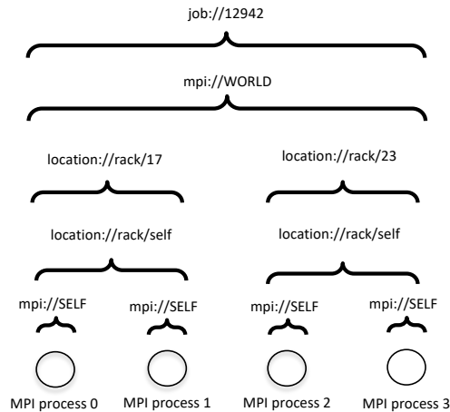
Figure 10.2: Examples of process sets. Illustrated are the two mandated process sets - mpi://WORLD and mpi://SELF - along with several optional ones that a runtime could define.
