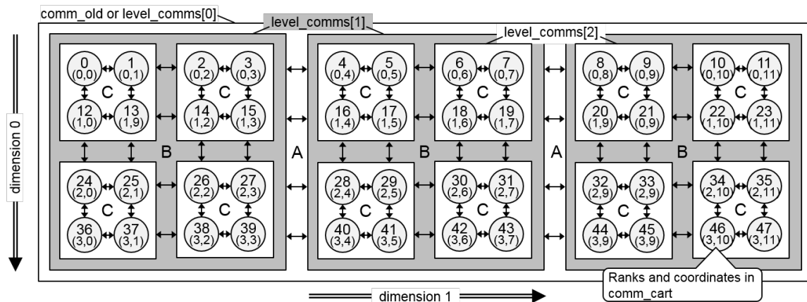
Figure 7.2: Example with a comm_old with 48 processes, ndims=2 , dim_weights=(1./4, 1./12) , and nsplit_types=2 and split_types , e.g., splitting into ccNUMA nodes and those into CPUs, and here with 4 cores per CPU and 4 CPUs per node. The level_comms[i] show this splitting of comm_old into hierarchical subcommunicators. The renumbering in comm_cart should first minimize the communication A (here, e.g., the communication between the ccNUMA nodes), then B (here, e.g., the CPU to CPU communication), and last C (here, e.g., the core to core communication)
