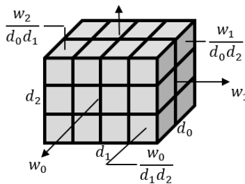
Figure 7.3: Communication model: The dim_weights[i]= w_i express the total communication cost in the direction of dimension i . The communication cost of one process in direction i is therefore w_i / \prod_{j,j \neq i} d_j with dims[i]= d_i .
