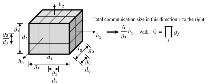
Figure 7.1: Example for the calculation of the weights. The data sizes g_i express the three dimensions of the total application data grid. The virtual process grid dimensions are expressed by d_i . The figure shows the dividing of the total application grid into its subdomains. The value h_i represents the halo width in a given direction when the 2-dimensional side of a subdomain is communicated to the neighbor process in that direction.
