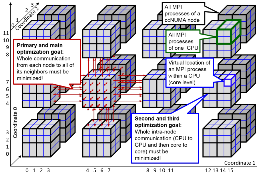
Figure 7.4: Example with 24 nodes (level 0), 4 CPUs per node (level 1) and 8 cores per CPU (level 2). The figure shows the 3-dimensional distribution calculated by MPI_DIMS_ML_CREATE based on weight values (1/12, 1/16, 1/8).
