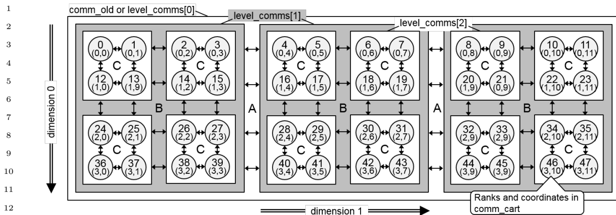
Figure 7.2: Example with a comm_old with 48 processes, ndims=2 , dim_weights=(1./4, 1./12) , and nsplit_types=2 and split_types , e.g., splitting into ccNUMA nodes and those into CPUs, and here with 4 cores per CPU and 4 CPUs per node. The level_comms[i] show this splitting of comm_old into hierarchical subcommunicators. The renumbering in comm_cart should first minimize the communication A (here, e.g., the communication between the ccNUMA nodes), then B (here, e.g., the CPU to CPU communication), and last C (here, e.g., the core to core communication)
