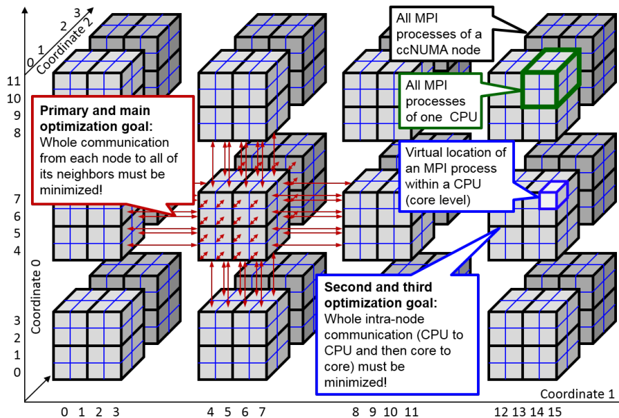
Figure 7.4: Example with 24 nodes (level 0), 4 CPUs per node (level 1) and 8 cores per CPU (level 2). The figure shows the 3-dimensional distribution calculated by MPI_DIMS_HW_CREATE_WEIGHTED based on weight values (1/12, 1/16, 1/8).
